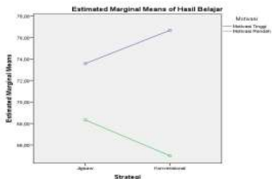
Gambar 1 Diagram Plot antar variabel
