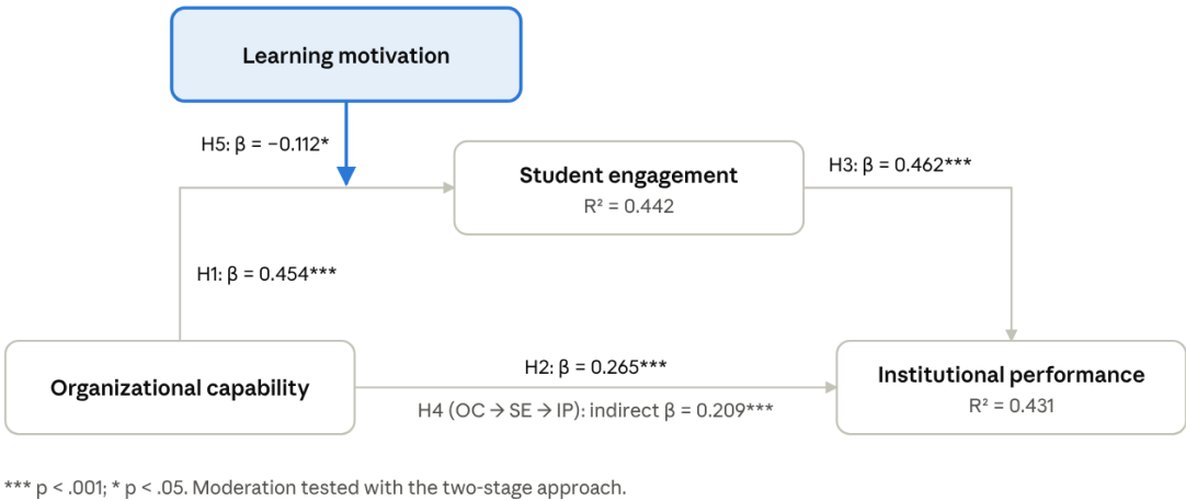
Figure 1. Research model with estimated paths (n = 218)
